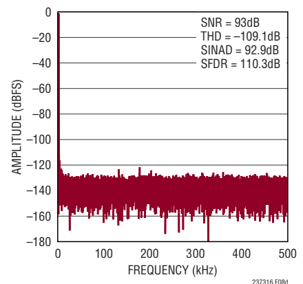
Figure 8d. 32k Point FFT f_{\text{SAMPL}} = 1\text{Msps} , f_{\text{IN}} = 1\text{kHz} for Circuit Shown in Figure 8a; Driven with Bipolar Inputs
