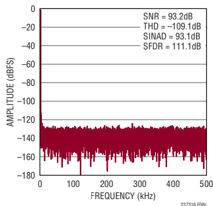
Figure 8c. 32k Point FFT f_{\text{SAMPL}} = 1\text{Msps} , f_{\text{IN}} = 1\text{kHz} for Circuit Shown in Figure 8a; Driven with Unipolar Inputs
