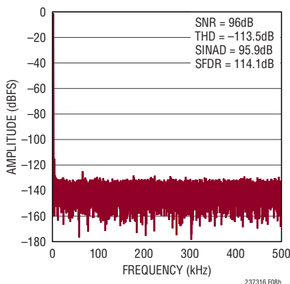
Figure 8b. 32k Point FFT f_{\text{SAMPL}} = 1\text{Msps} , f_{\text{IN}} = 1\text{kHz} for Circuit Shown in Figure 8a; Driven with Fully Differential Inputs
