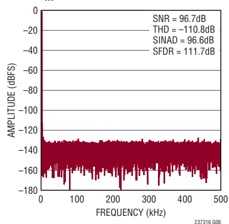
32k Point FFT f_{SAMPL} = 1\text{Mps} , f_{IN} = 1\text{kHz} , REF_{BUF} = 5\text{V}
